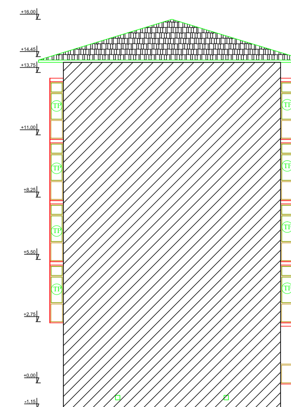
FATADA LATERALA STANGA PROPUS
