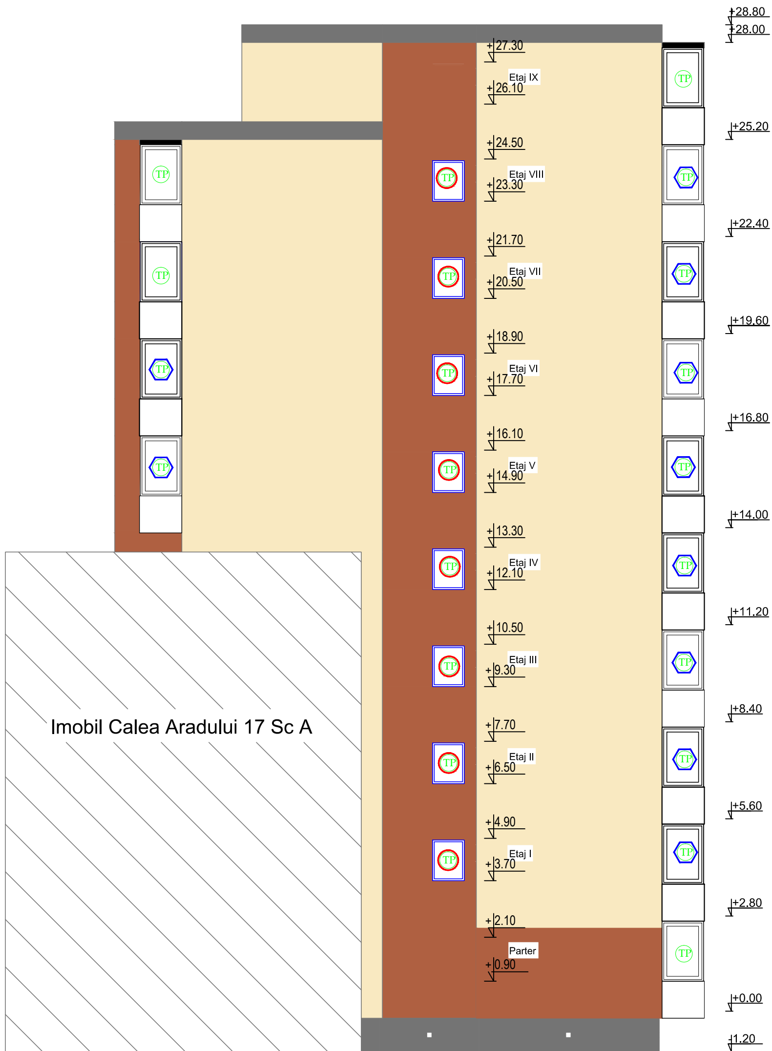
Fatada lateral stanga propusa Scara 1:100
