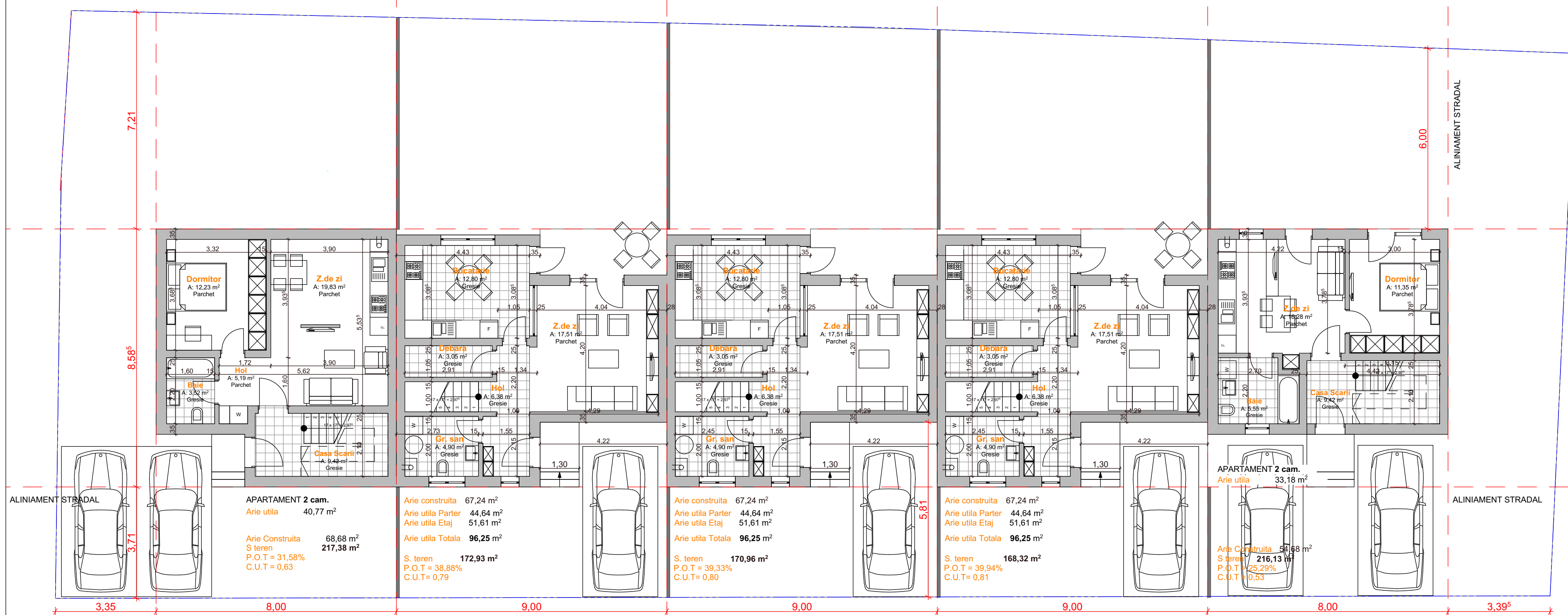
Planuri PARTER, Sc.1:200
