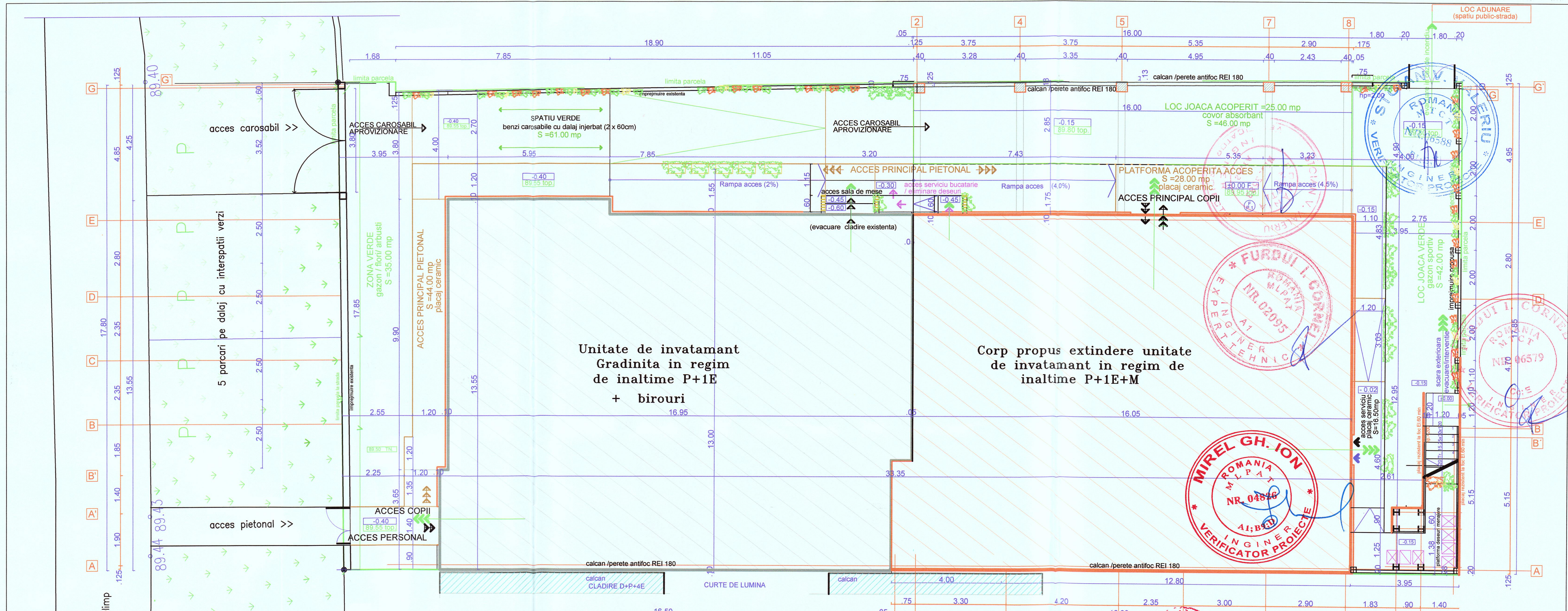
PLAN AMENAJARE PARCELA Sc.1:100
