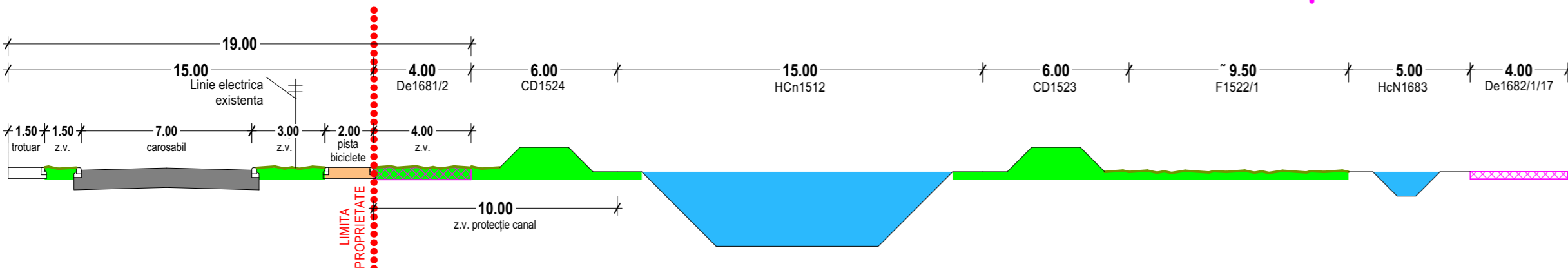
PROFIL TRANSVERSAL TIP PTT1 - DRUM COLECTOR PROPUȘ
